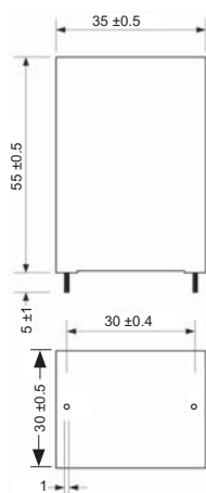
Specifications casing 1: Bucket: Plastic bucket UL 94-V0 Terminals: copper wire, tin-plated Ø1.0 mm Weight: approx. 70g
